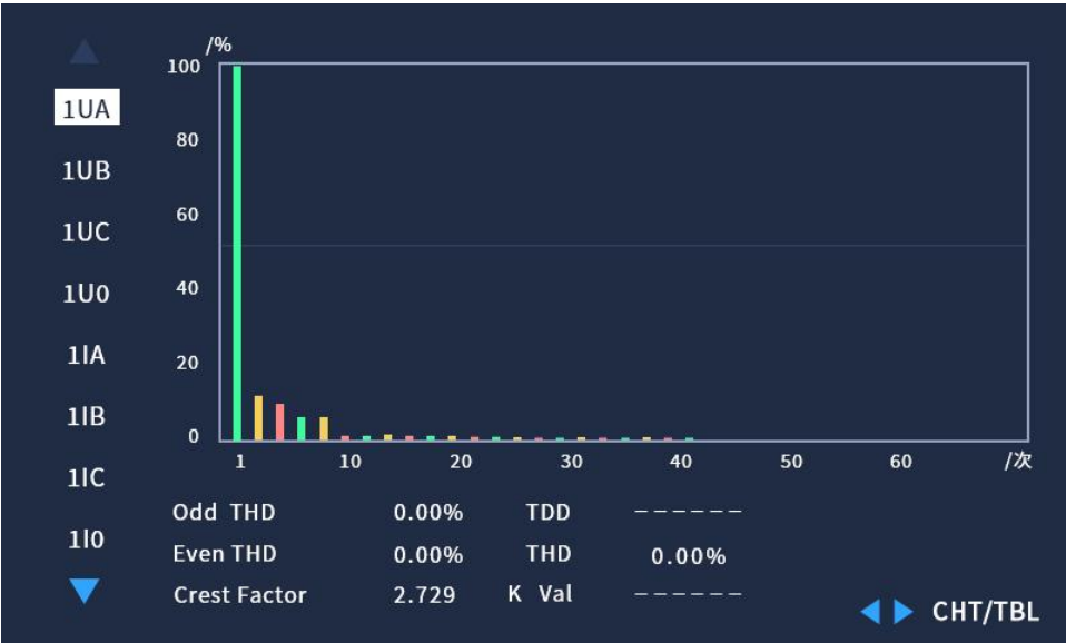
Fig. 4.13 Harmonics Chart
