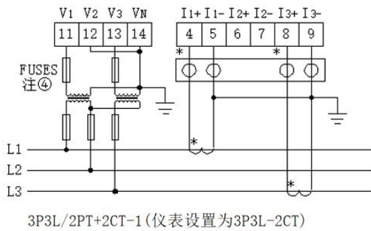
3P3L/2PT+2CT-1 (仪表设置为3P3L-2CT)
