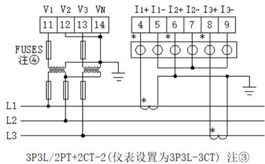
3P3L/2PT+2CT-2 (仪表设置为3P3L-3CT) 注③
